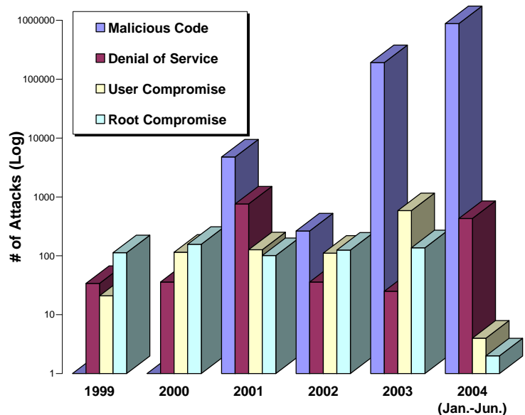
US-CERT data on Hacker incidents by type
